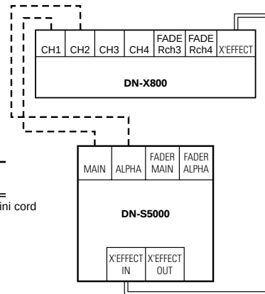
Fig. 2 : X-Effect connections example 1
