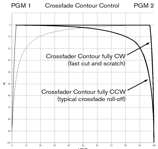
Figure 3. Crossfader Contour control
