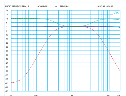
Figure 1. PGM Bass & Treble Controls
