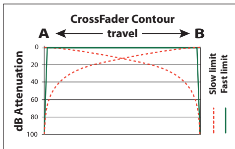
Figure 3. Crossfader Contour control
